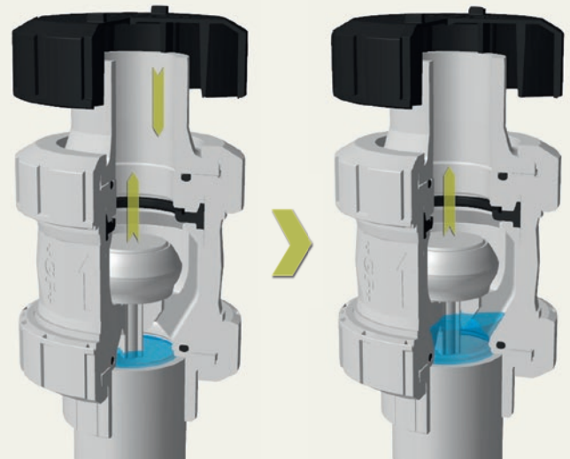
Valve open
